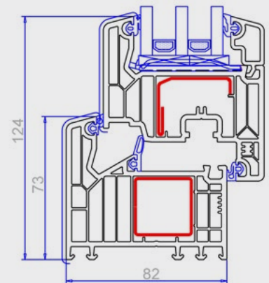
↑ Window Acryl-Color COEX
