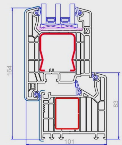
↑ Door Acryl-Color COEX
