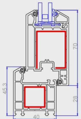
↑ Door standard
