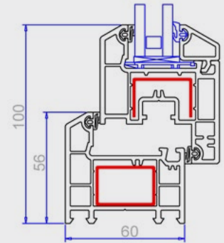
↑ Window standard
